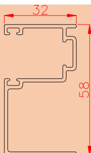
TK1438 Guide with great shoulder Weight 0,670 kg/m
