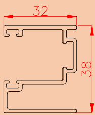
TK1436 Guide with small shoulder Weight 0,590 kg/m
