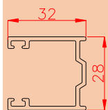
TK1431 Single guide Weight 0,320 kg/m
